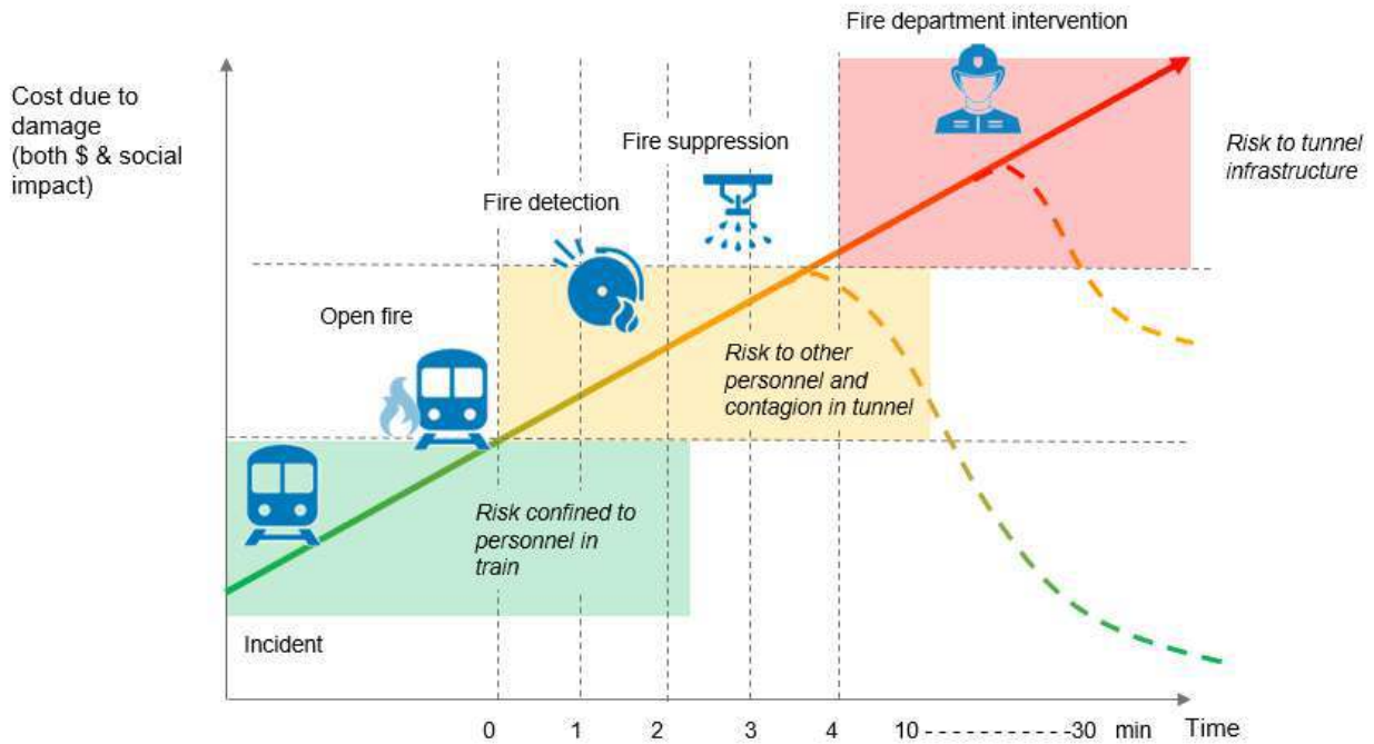
Figure 1 - Progression of tunnel fire with time
