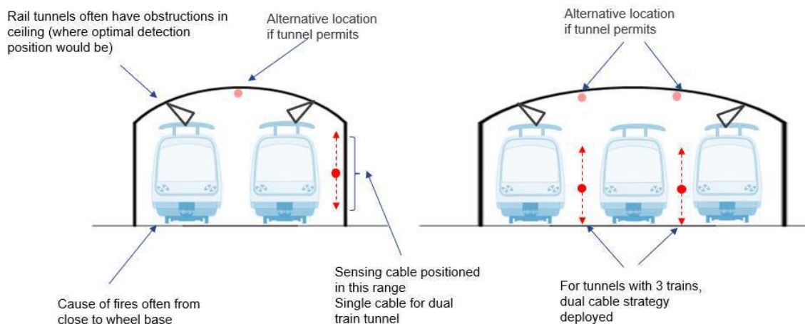
Figure 7 - Single and dual cable configurations
