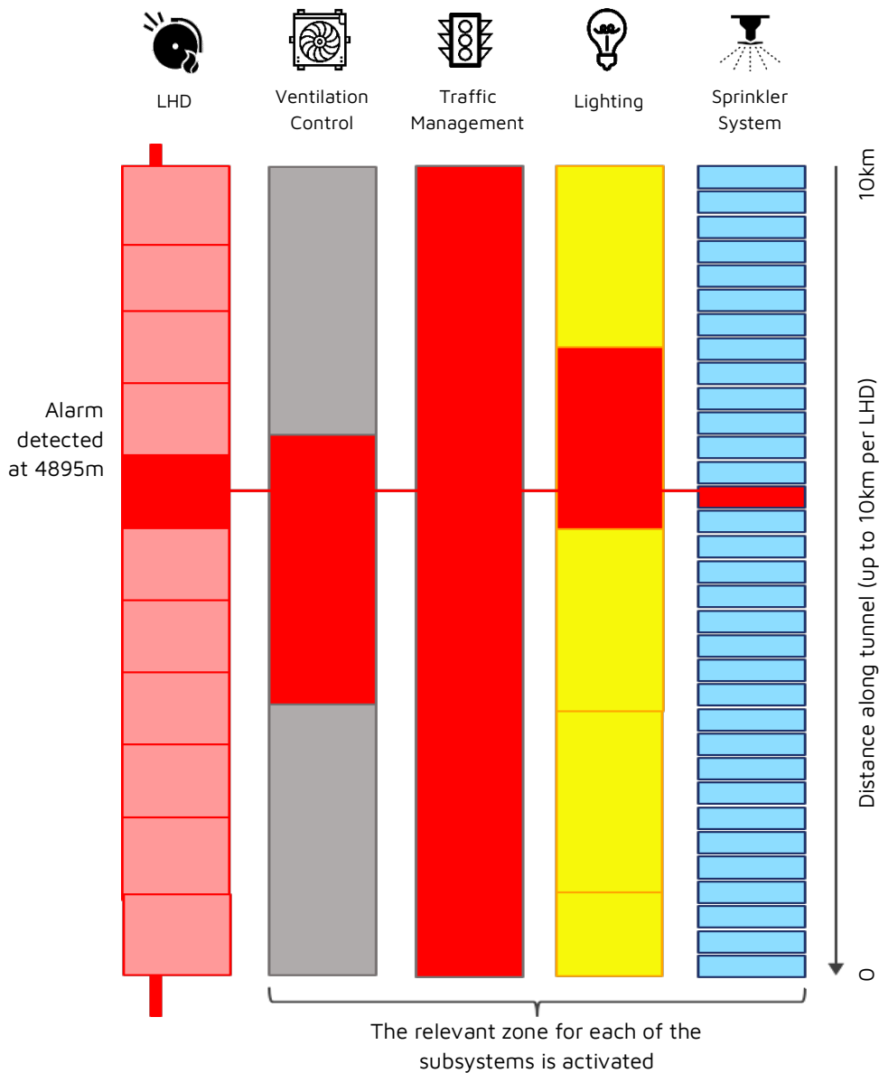
Figure 5 - Example of smart zone configuration
