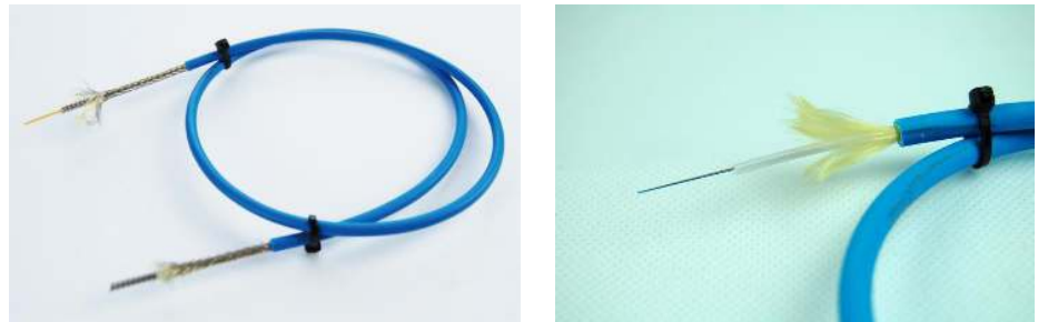
Figure 6- Examples of FireFiber cables
