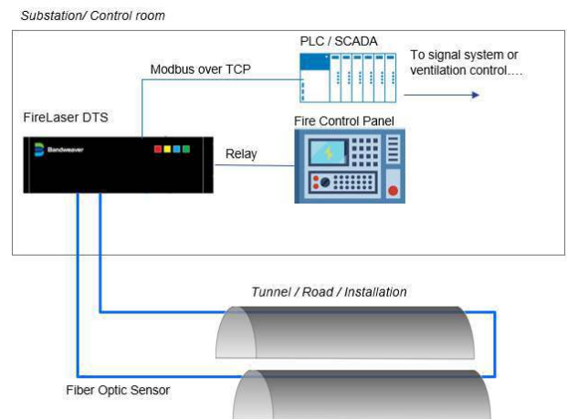
Figure 4 - Example of System Architecture
