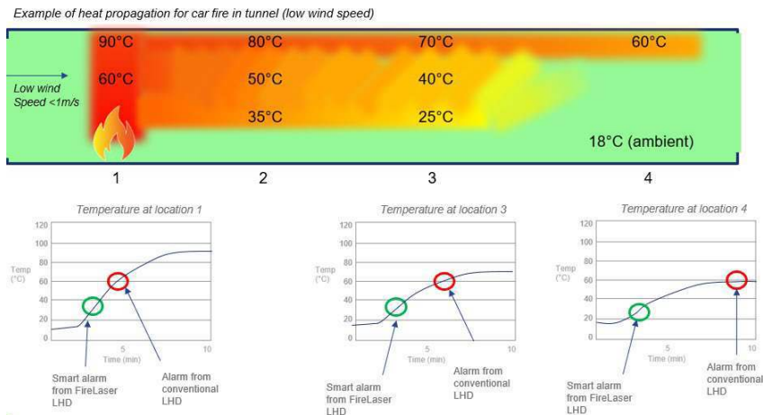
Figure 3 - Temperature profile of tunnel fire
