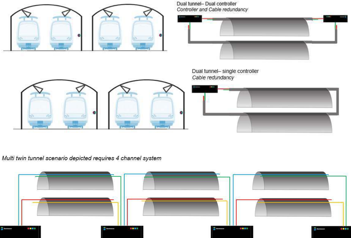
Figure 9 - System redundancy options
